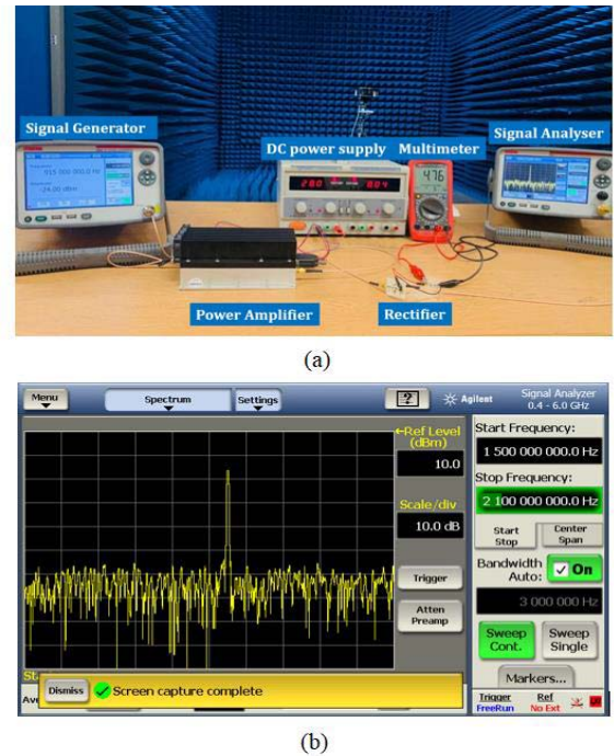
Fig. 16. (a) Experimental setup for rectifier measurement. (b) Harmonic spectrum at 12-dBm input power.
