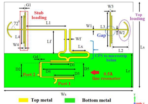
Fig. 2. Proposed duplexing antenna.
