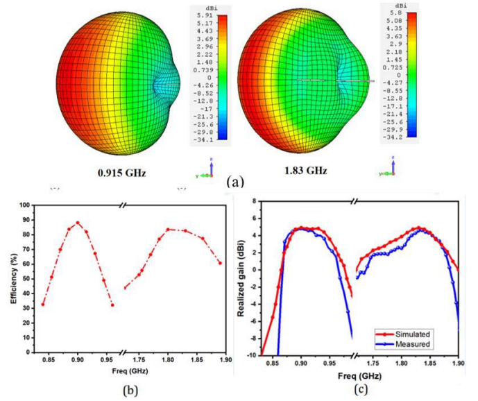
Fig. 9. (a) Simulated 3-D radiation patterns with excitation at ports 1 and 2, respectively. (b) Simulated efficiency. (c) Realized gain of duplexing antenna.
