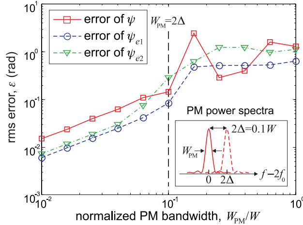
Fig. 3. Rms error of even phase functions \psi_{e1} (circles), \psi_{e2} (triangles), and complete phase \psi (squares) versus normalized PM bandwidth at fixed PM spacing of 2\Delta = 0.5 THz. Inset shows the definition of PM power spectral pair used in the simulation.
