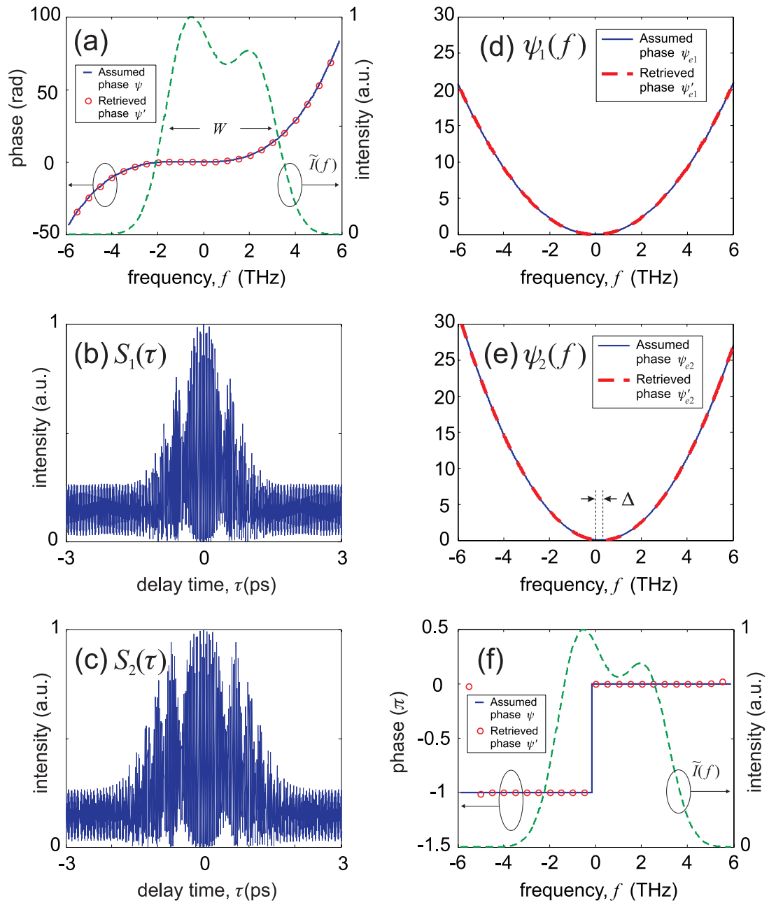
Fig. 2. Theoretical verification of MIFA method. (a) Assumed power spectrum (dash), assumed spectral phase (solid), retrieved spectral phase (open circles). (b-e) The corresponding MIFA traces S_1(\tau) , S_2(\tau) , and even phases \psi_{e1}(f) , \psi_{e2}(f) produced in retrieving spectral phase in (a). (f) Simulation result by assuming \pi -phase shift. The corresponding rms errors in (a) and (f) are 8.18 \times 10^{-5} rad, and 6.13 \times 10^{-5} rad, respectively.
