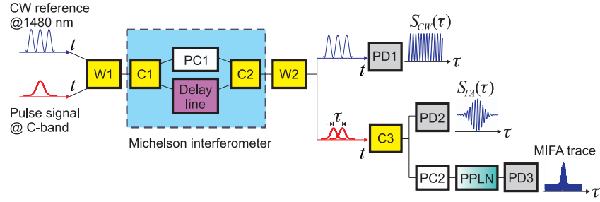
Fig. 4. Experimental setup of MIFA measurement. W#: WDM, C#: 3-dB coupler, PC#: polarization controller, PD1&PD2: InGaAs photodetectors, PD3: Si photodetector.
