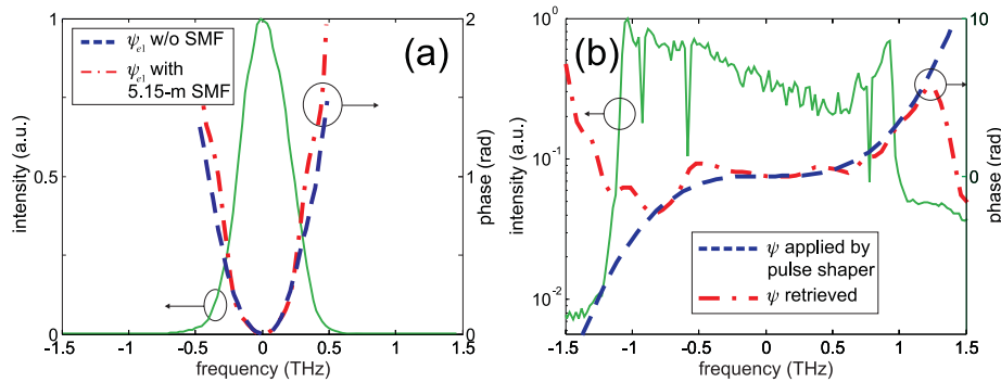
Fig. 5. (a) Even-order spectral phase before (dash) and after (dash-dot) the insertion of 5.15-m-long SMF. (b) Complete spectral phase imposed by pulse shaper (dash) and retrieved by MIFA scheme (dash-dot).
