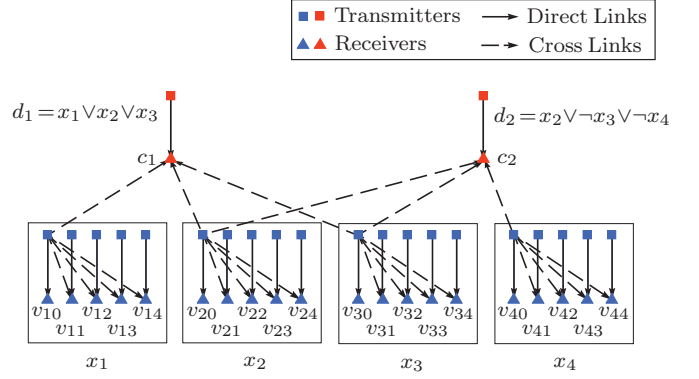
Fig. 1. Illustration of the correspondence between a 3-SAT problem instance (x_1 \vee x_2 \vee x_3) \wedge (x_2 \vee -x_3 \vee -x_4) , which consists of N = 4 Boolean variables and M = 2 clauses, and a MISO IFC with K = 5 \times 4 + 2 pairs of transmitters and receivers.
