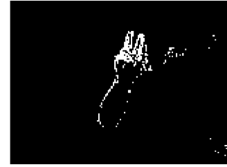
Fig. 6. The combined region C_i(x, y) .
