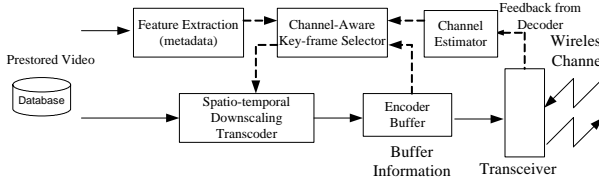
Fig. 1. Proposed streaming server architecture.
