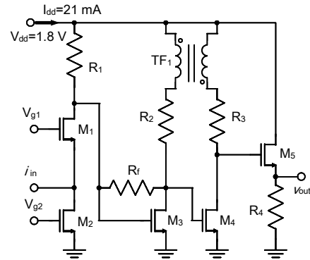
Fig. 1 Schematic of the TIA with transformer peaking.
