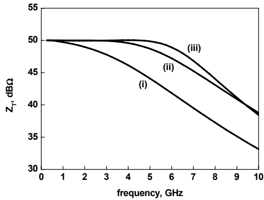
Fig. 2 Simulated Z_T versus frequency for the TIA with (i) resistive load (ii) inductor peaking (iii) transformer peaking.
